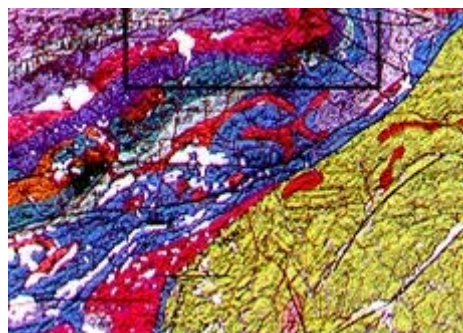
Geological map and SAR data integrated
